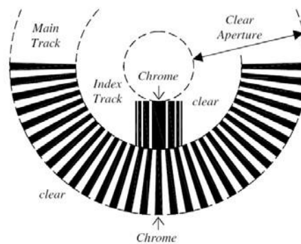
Figure 1b: Rotary Grating Pattern Layout
