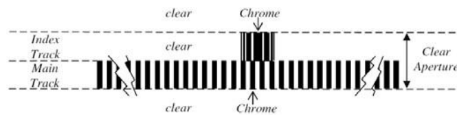
Figure 1a: Linear Grating Pattern Layout
