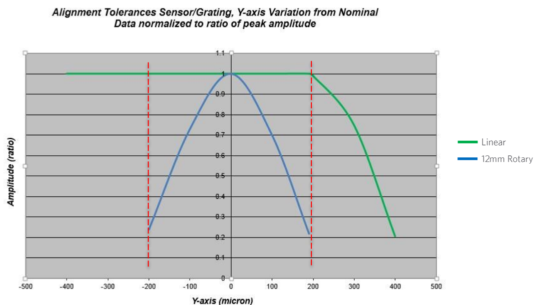
Figure 3: Y alignment tolerance study
